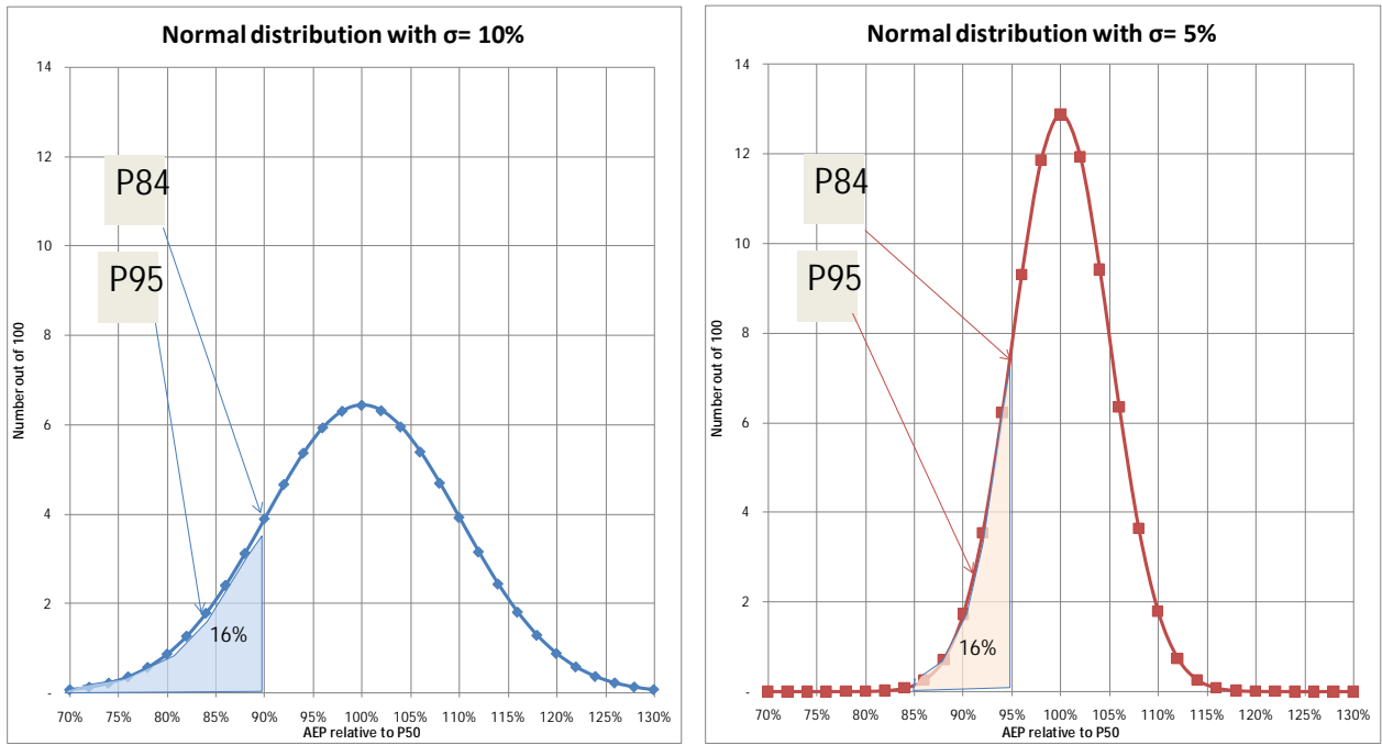
Figure 2 The Normal distribution is defined so that roughly 2/3 (more precisely 68,3%) of all events will be within +/- \sigma and around 32% is outside. In the one tail (e.g. below -\sigma ), there is around 16%, so there is 16% probability that the estimate will be below 1\sigma subtracted from P50, or 84% probability that it will be above (exceed). In other words, the P84 is the value where 84 out of 100 realizations will result in an outcome better than P84. For P95, there is only 5% probability to get an outcome poorer than this exceedance level which is found by subtracting the \sigma multiplied by 1,64 from the P50. So for \sigma=10\% , the P95 value in the left graph where 5% would be “in the shaded area” (P95), would be found 16,4% below 100%, i.e. at 83,6% on the x-axis. Similarly, if \sigma=5\% , 5\% \times 1,64 = 8,2\% , so P95 is found at AEP of 100\%-8,2\% = 91,8\% of the P50 on the x-axis.
