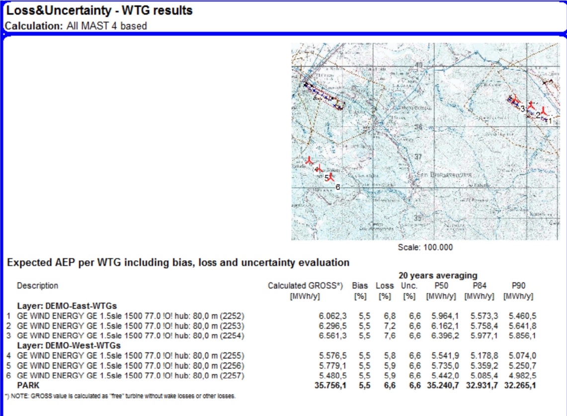
Figure 24 This page show results turbine by turbine, thereby the needed details for projects sold turbine by turbine are available.
