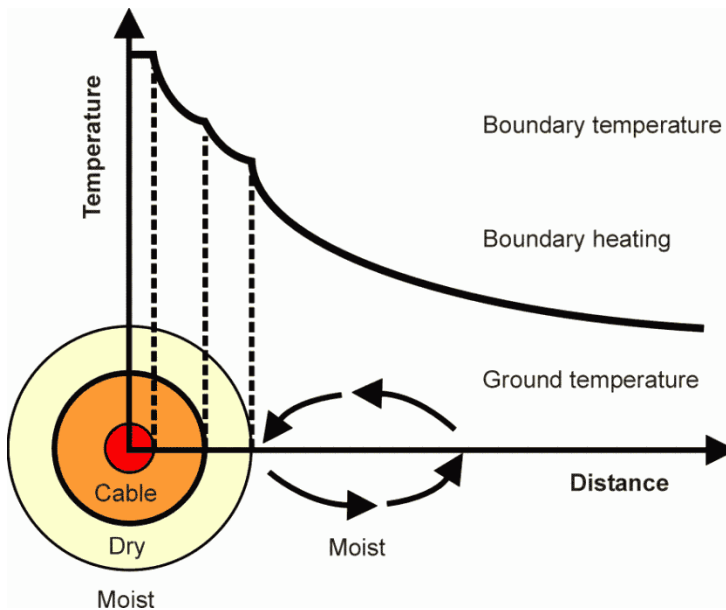
Figure 23 The cables heat up the near surroundings making this a dry area, which influences the transportation of heat from the cable.
