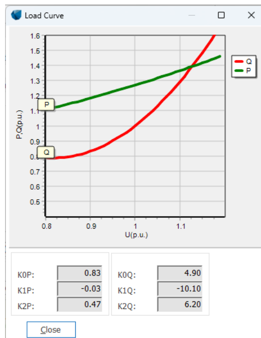
Figure 15 Presentation of voltage dependent Load Characteristic
