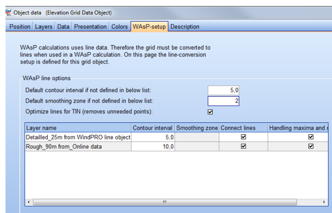
Figure 5 - Setting elevation data in a elevation grid object
