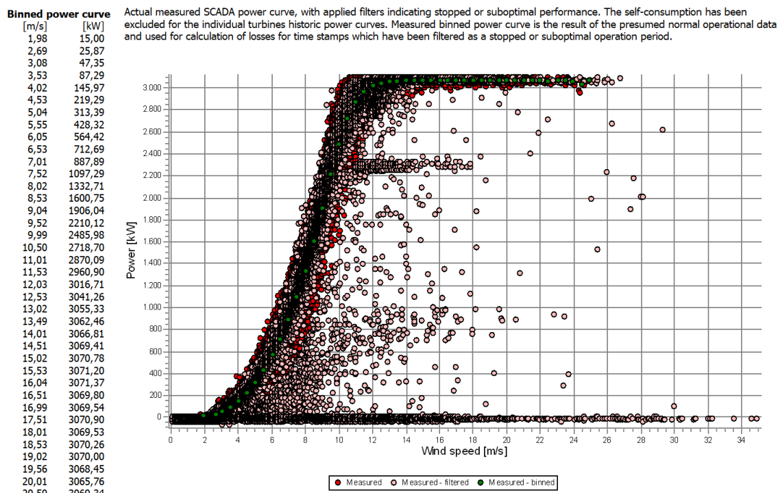
Figure 65: Example historic power curve based on the nacelle wind speed.
