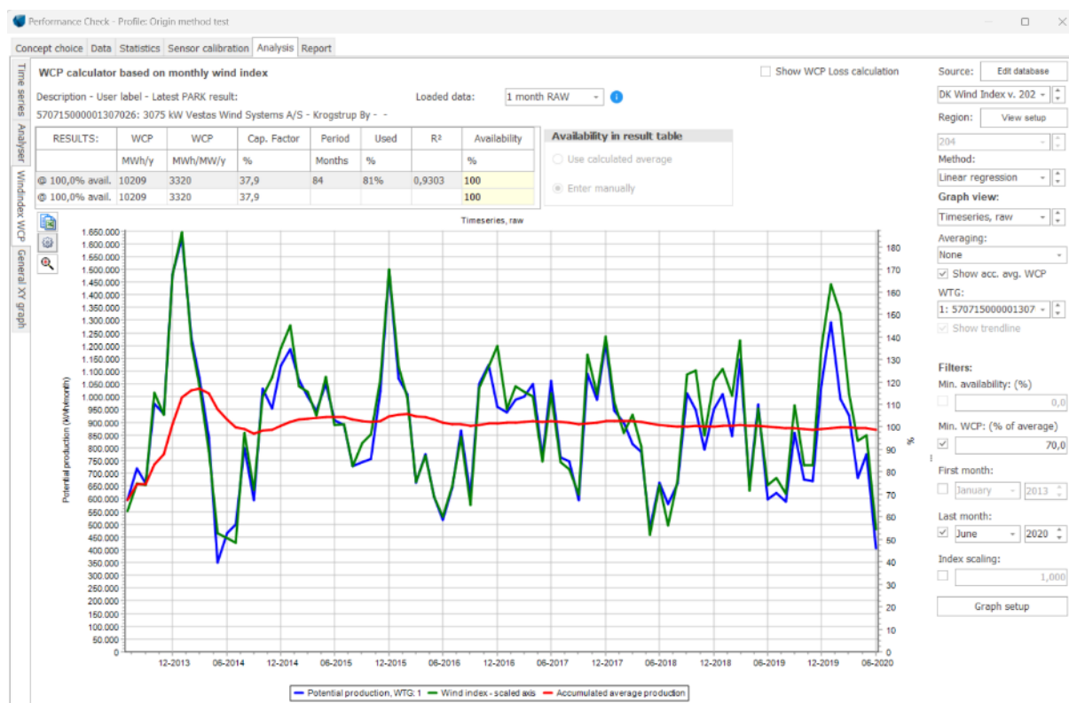
Figure 75 Normalized monthly production data.
