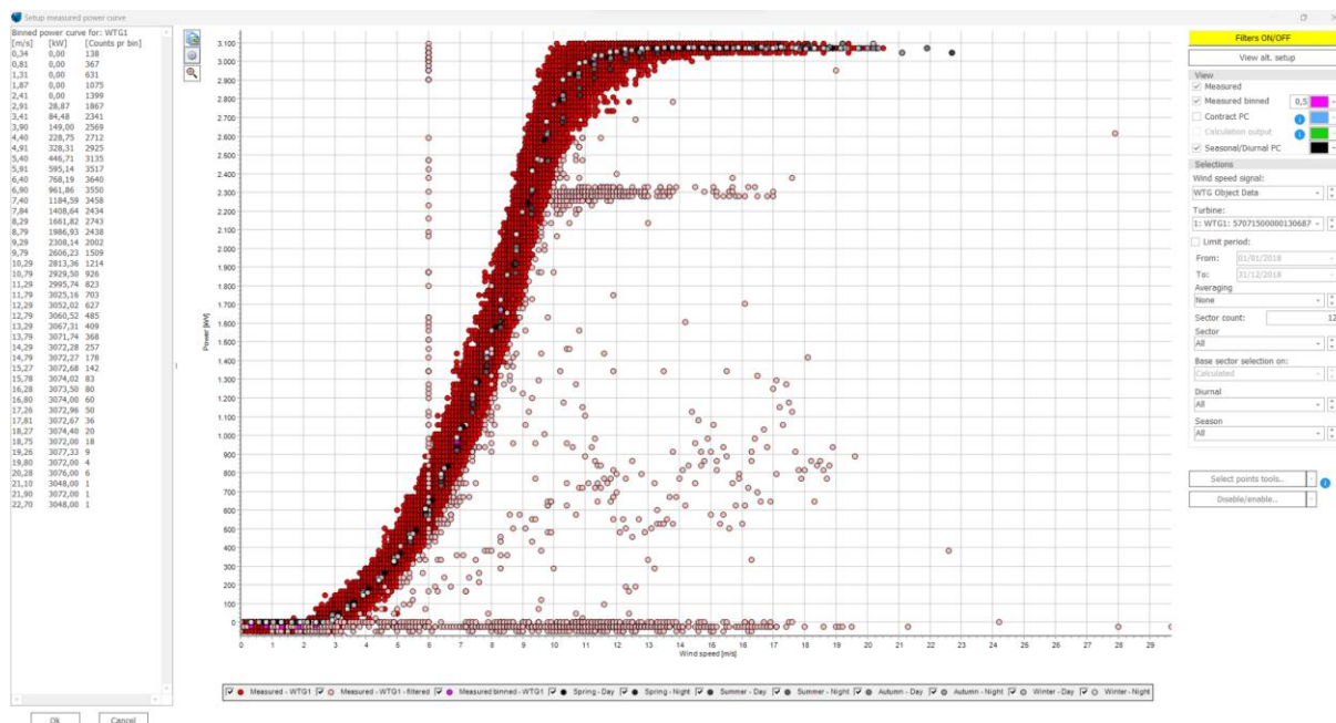
Figure 48: Historic power curve
