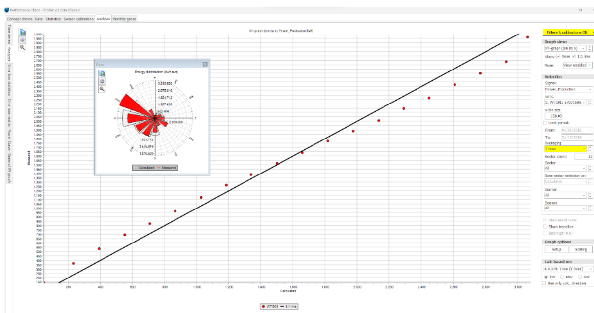
Figure 89 Binned calculated power vs measured for model validation.
