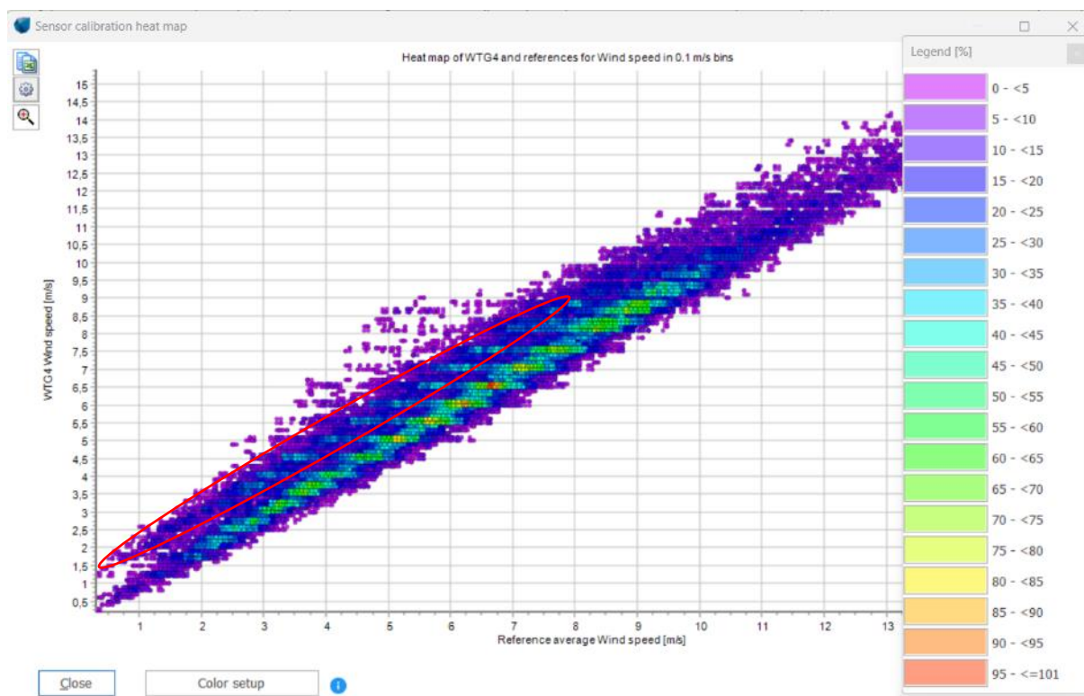
Figure 42: Heat map of reference versus individual wind speed
