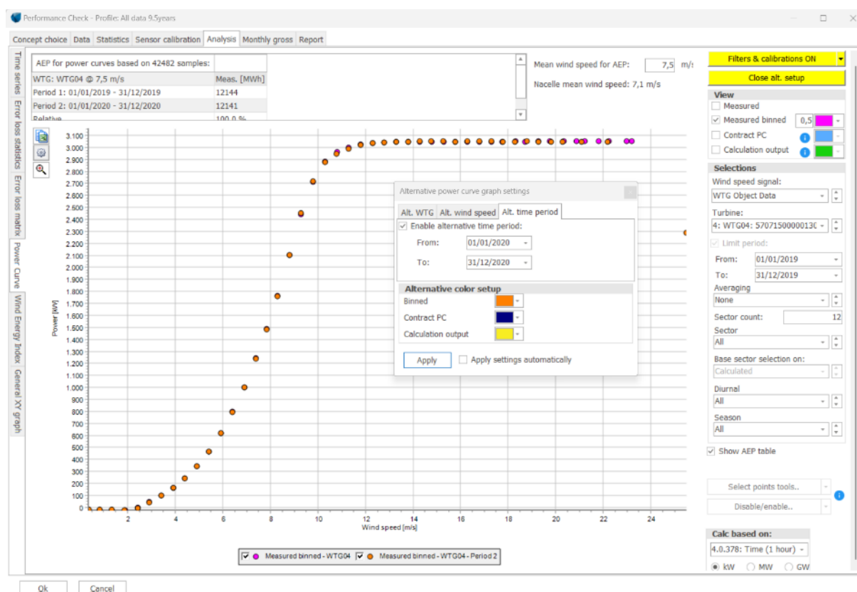
Figure 86 Two periods binned power curves plot.
