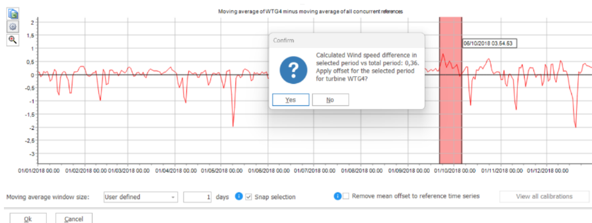
Figure 43: Example of inconsistent nacelle wind speed
