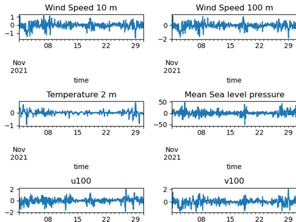
Figure 13: November 2021: Time series of differences between ERA5T and ERA5 for a location in the North Sea (latitude=55, longitude=8). Wind speed differences in m/s, pressure differences in Pa, temperature differences in C.
