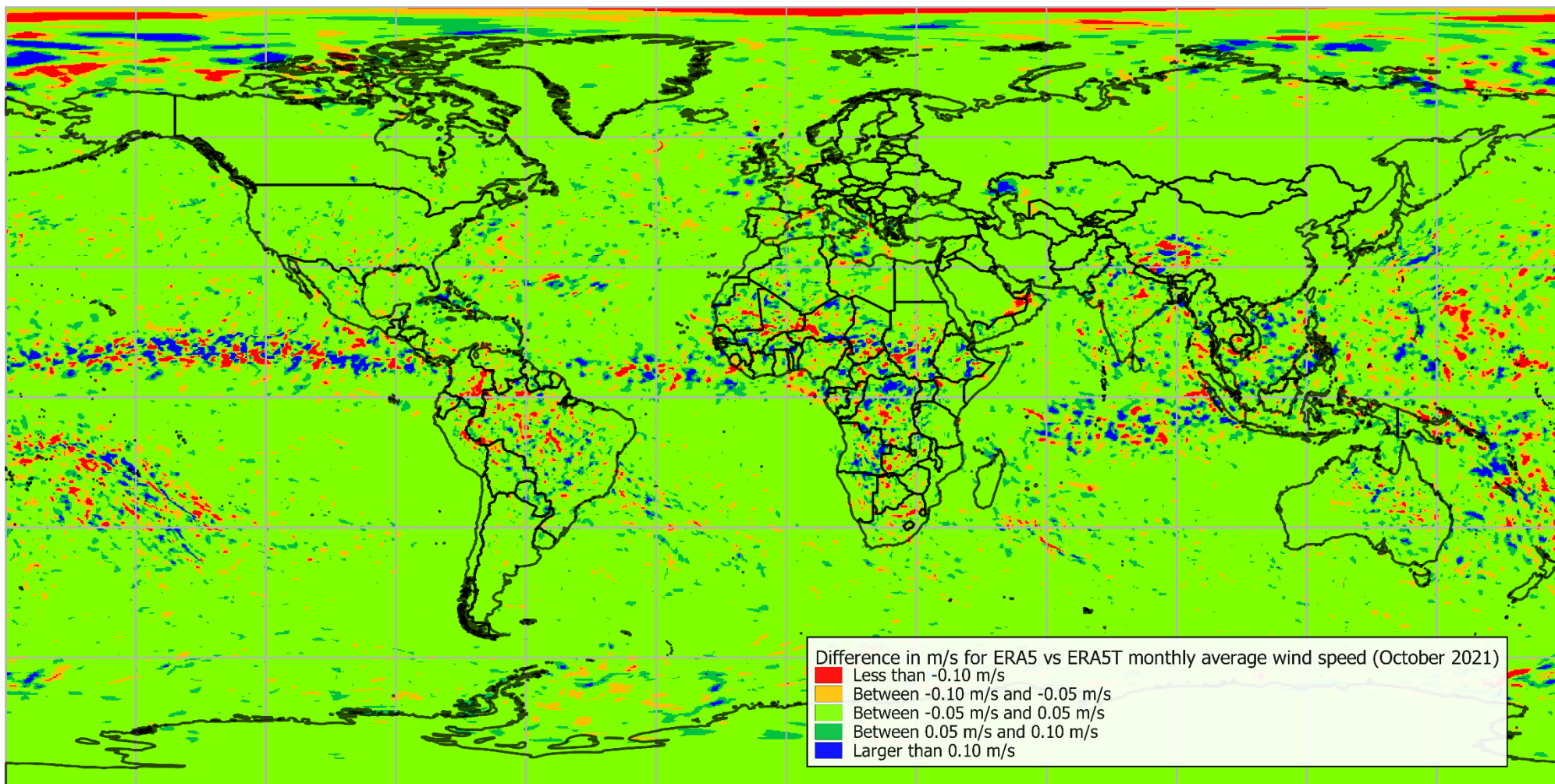
Figure 2: October 2021: Absolute deviation [m/s] between ERA5 and ERA5T for monthly average wind speeds at 100m.
