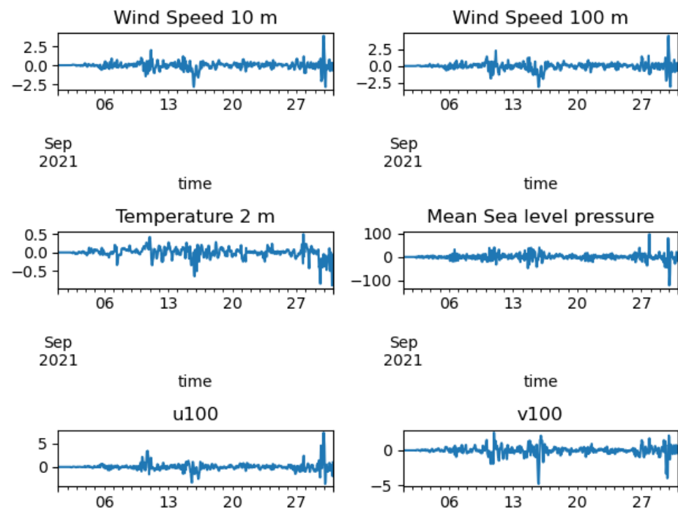
Figure 9: September 2021: Time series of differences between ERA5T and ERA5 for a location in the North Sea (latitude=55, longitude=8). Wind speed differences in m/s, pressure differences in Pa, temperature differences in C.
