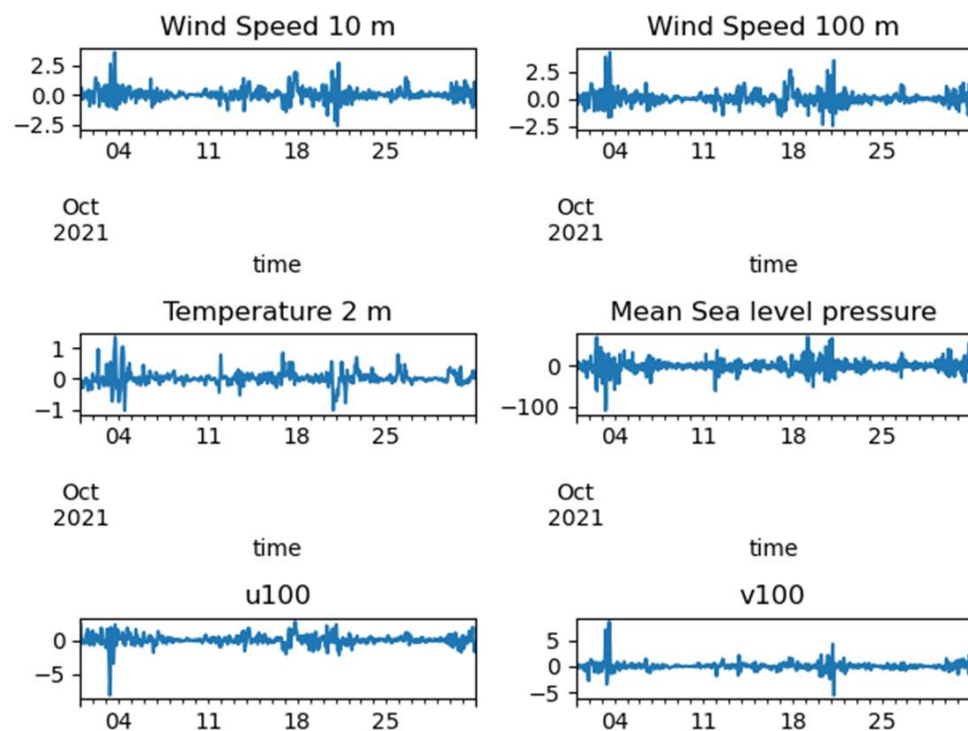
Figure 11: October 2021: Time series of differences between ERA5T and ERA5 for a location in the North Sea (latitude=55, longitude=8). Wind speed differences in m/s, pressure differences in Pa, temperature differences in C.
