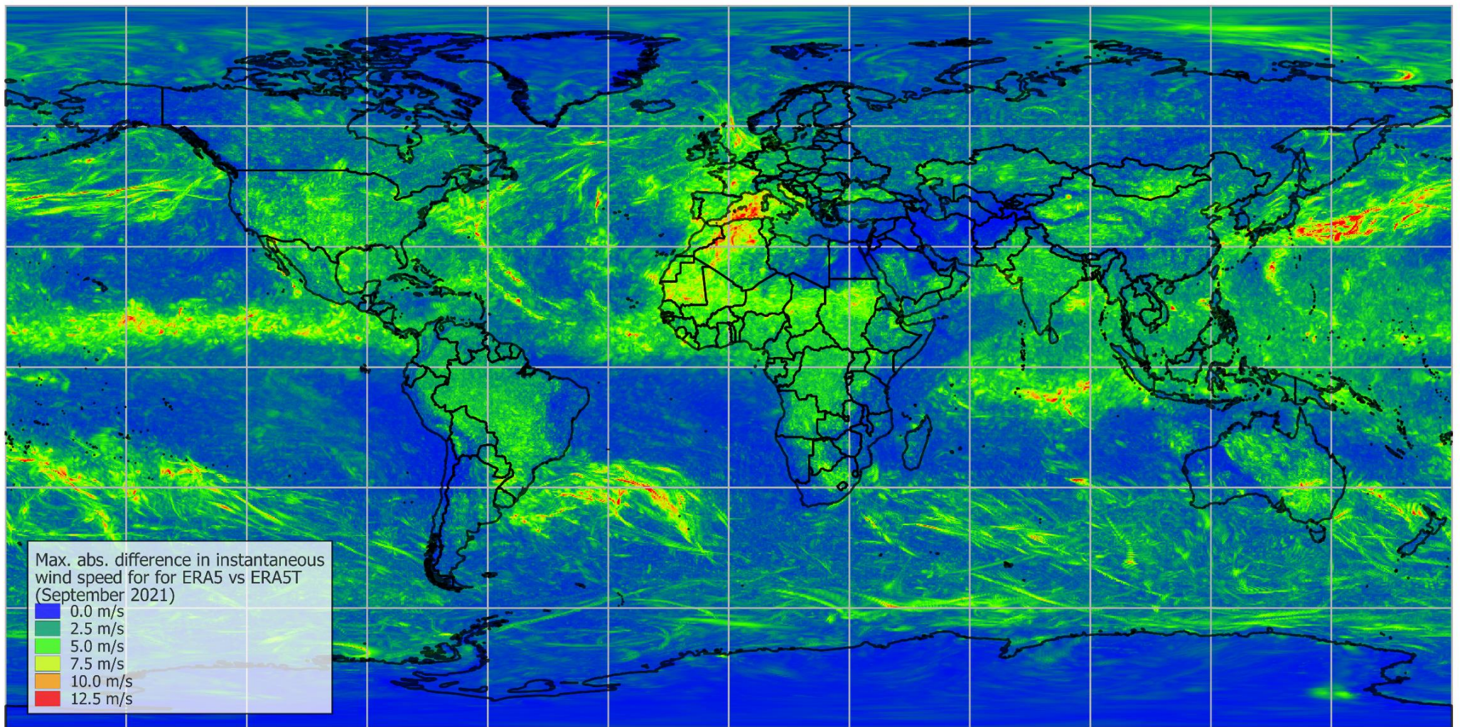
Figure 14: September 2021: Maximum absolute difference in instantaneous wind speed (individual hourly time-series samples) for ERA5 vs ERA5T. Parameter: 100m wind speeds.
