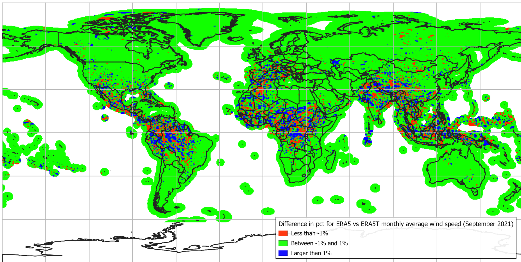
Figure 4: September 2021: Relative deviation [%] between ERA5 and ERA5T for monthly average wind speeds at 100m.
