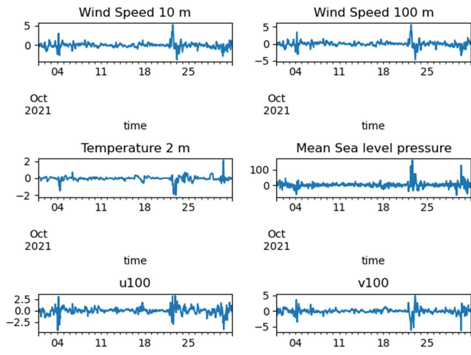
Figure 10: October 2021: Time series of differences between ERA5T and ERA5 for a location in the Western Mediterranean Sea (latitude=38, longitude=4). Wind speed differences in m/s, pressure differences in Pa, temperature differences in C.
