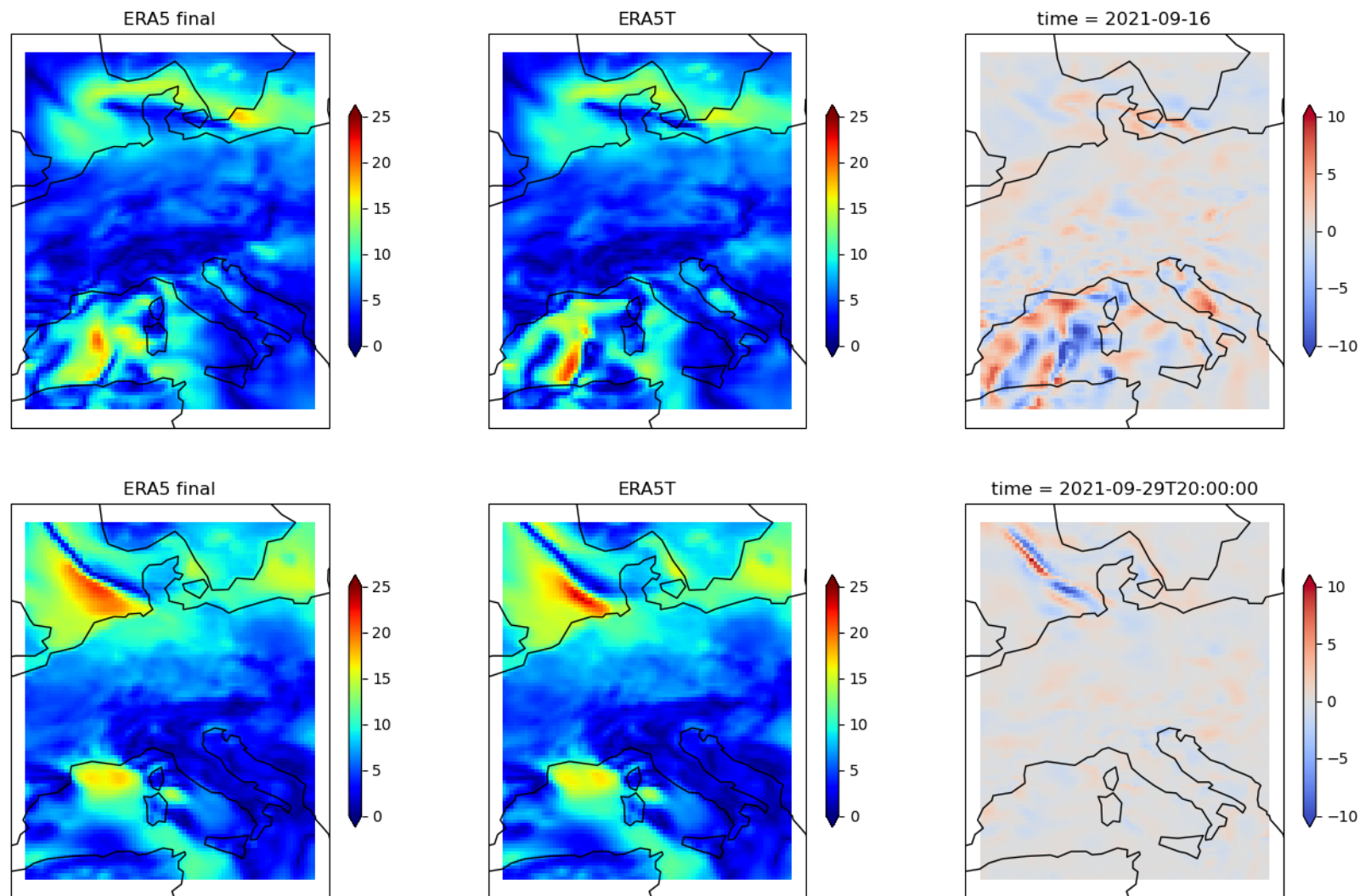
Figure 7: Two example time stamps (each row represents a time stamp) showing the validated final ERA5 data (left), the preliminary ERA5T (mid) and their difference (right). Parameter: 100m wind speeds.
