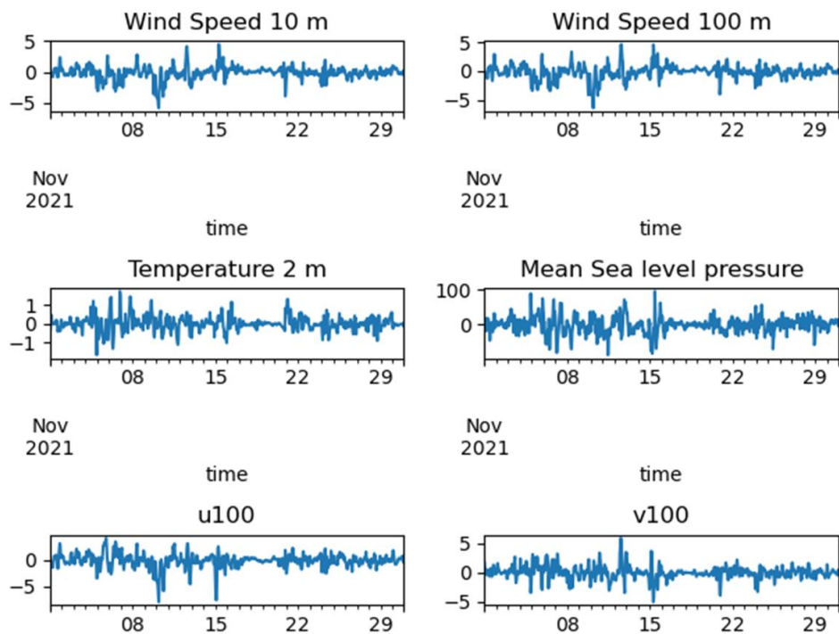
Figure 12: November 2021: Time series of differences between ERA5T and ERA5 for a location in the Western Mediterranean Sea (latitude=38, longitude=4). Wind speed differences in m/s, pressure differences in Pa, temperature differences in C.
