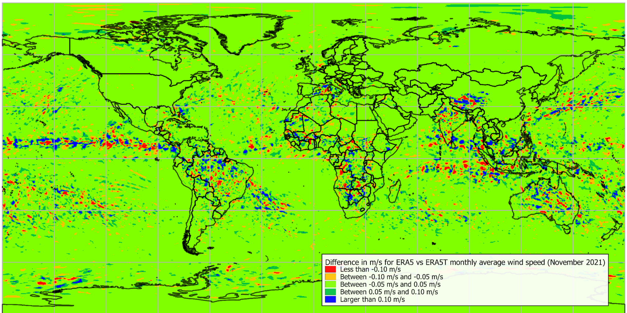
Figure 3: November 2021: Absolute deviation [m/s] between ERA5 and ERA5T for monthly average wind speeds at 100m.
