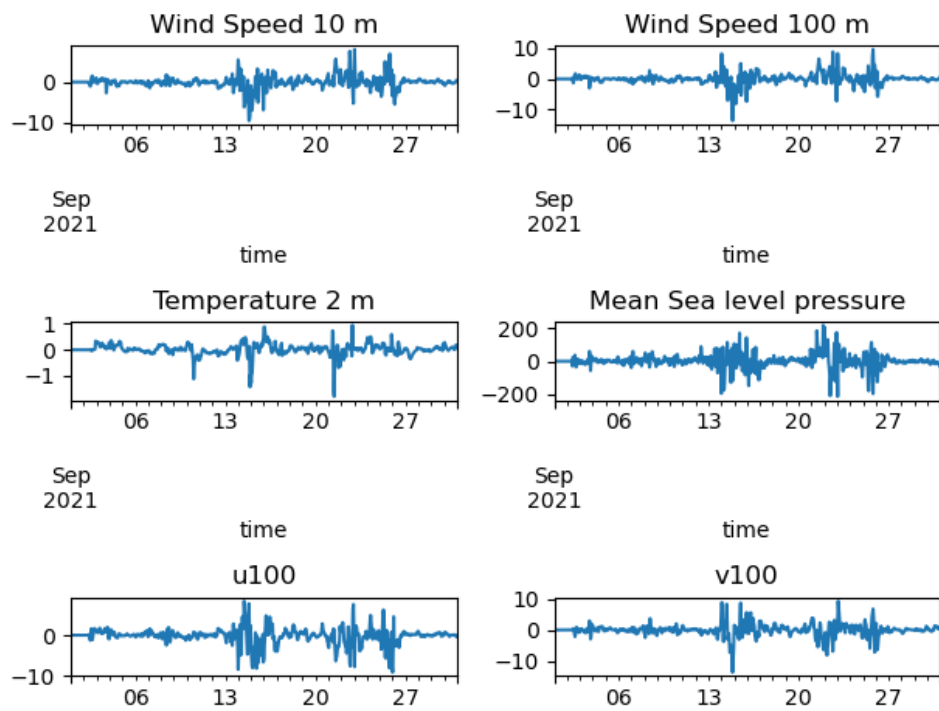
Figure 8: September 2021: Time series of differences between ERA5T and ERA5 for a location in the Western Mediterranean Sea (latitude=38, longitude=4). Wind speed differences in m/s, pressure differences in Pa, temperature differences in C.
