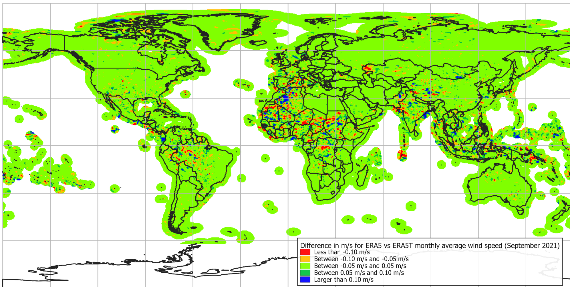
Figure 1: September 2021: Absolute deviation [m/s] between ERA5 and ERA5T for monthly average wind speeds at 100m.
